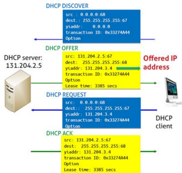
Figure 8: DHCP Procedure
